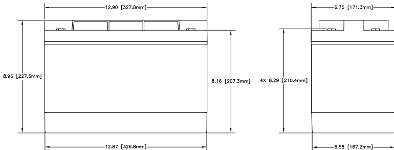
ENVELOPE DRAWING
